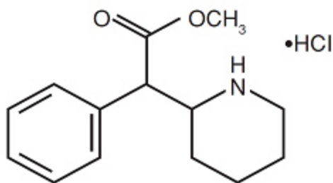
Figure 1. Methylphenidate HCl structure
