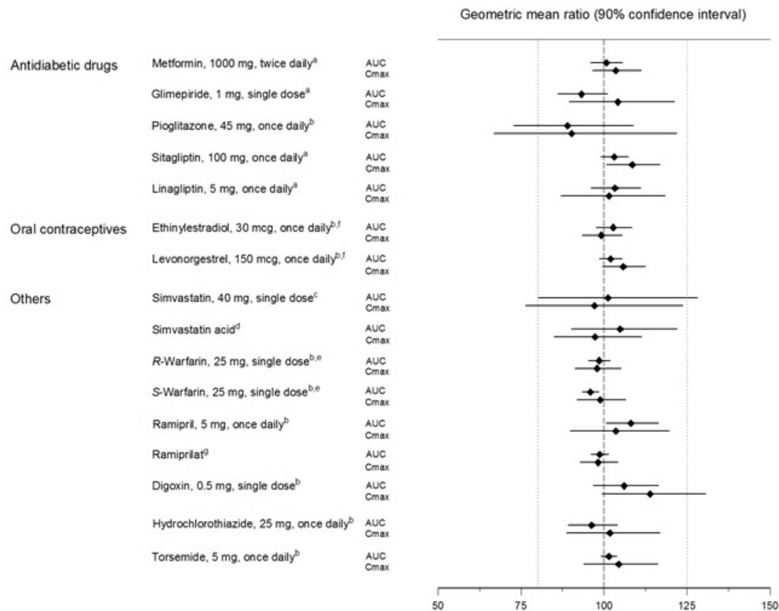
Figure 2 Effect of Empagliflozin on the Pharmacokinetics of Various Medications as Displayed as 90 % Confidence Interval of Geometric Mean AUC and C max Ratios [reference lines indicate 100 % (80 % - 125 %)]
